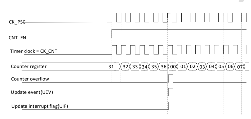
Figure 19-4 Counter timing diagram, internal clock divided by 1
