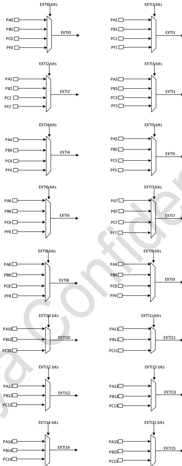
Figure 12-2 External interrupt/event GPIO mapping
