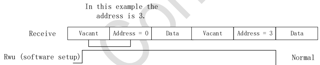
Figure 30-8 Silent mode with address tag detection
