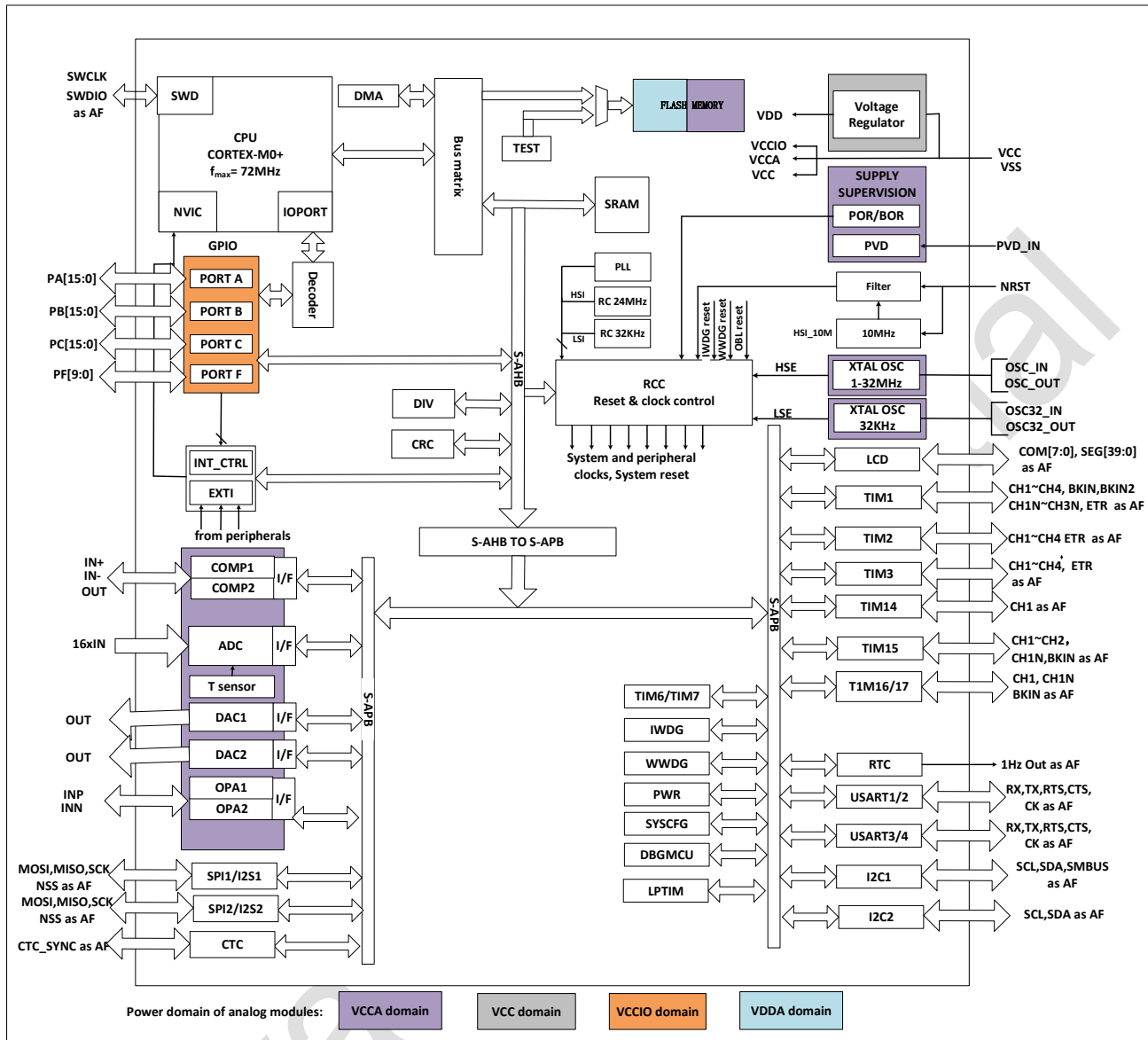
Figure 2-1 System architecture
