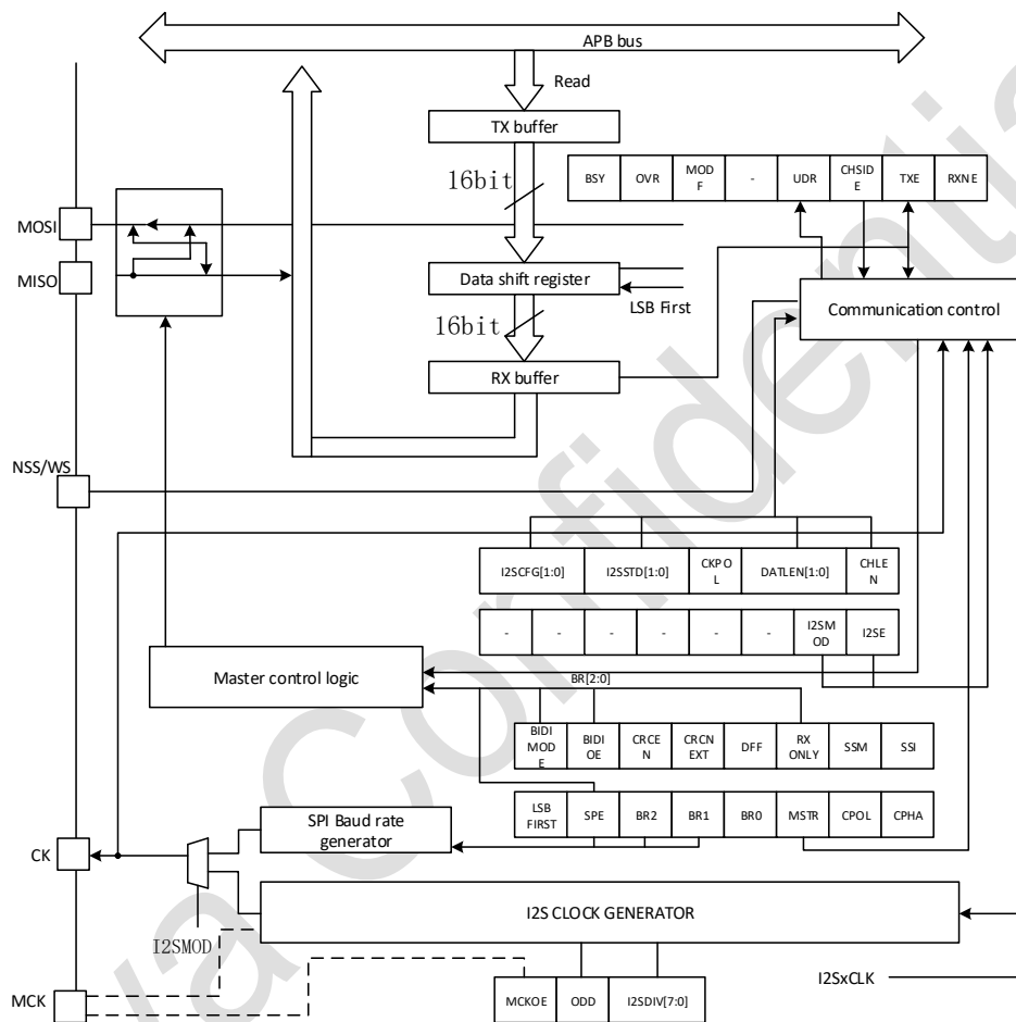
Figure 29-10 IIS Block Diagram
