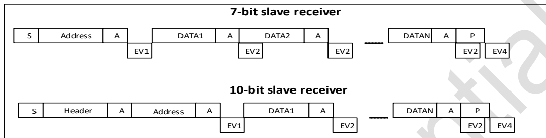
Figure 28-4 Slave receiver transmission sequence diagram
