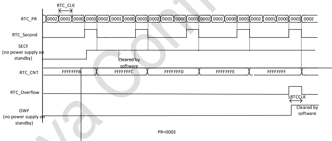
Figure 27-3 RTC overflow waveform example, PR = 0003
