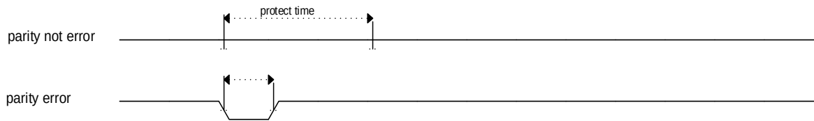
Figure 30-16 ISO7816-3 asynchronous protocol
