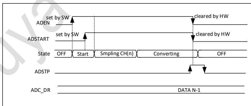
Figure 14-2 Stop timing
