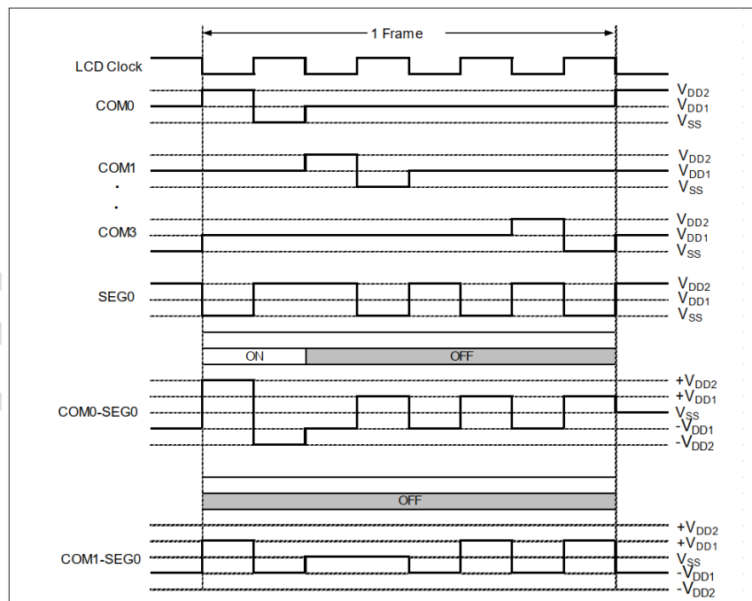
Figure 15-7 1/4Duty 1/2Bias Drive waveforms
