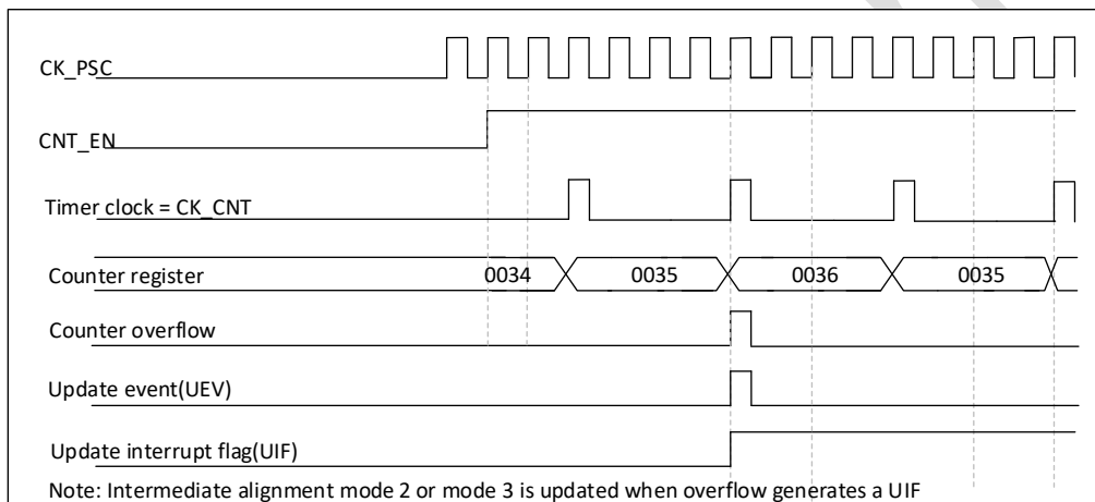
Figure 23-18 Counter timing diagram, internal clock divided by 4, TIMx\_ARR = 0x36
