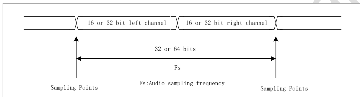
Figure 29-33 Audio Sample Definition
