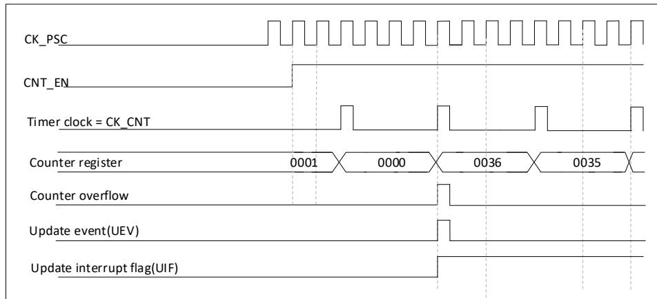
Figure 19-12 Counter timing diagram, internal clock divided by 4
