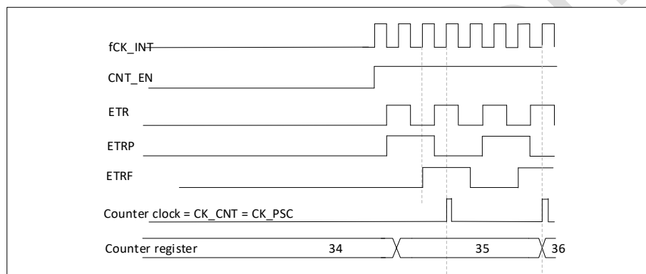
Figure 19-26 Control circuit in external clock mode 2
