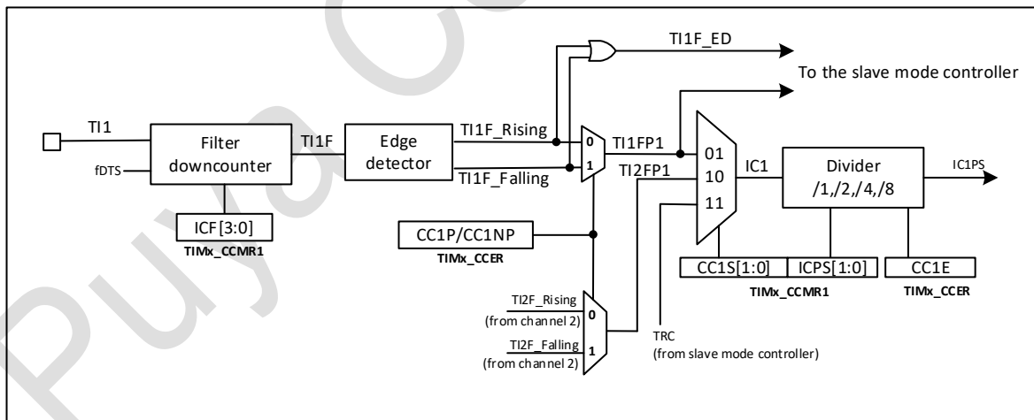
Figure 20-24 Capture/compare channel (example: channel 1 input stage)
