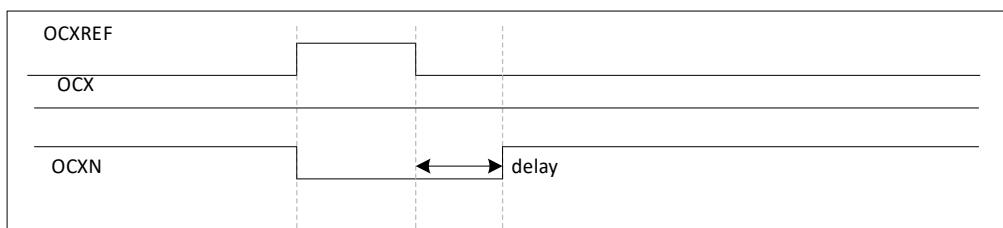
Figure 23-36 Dead-time waveforms with delay greater than the positive pulse
